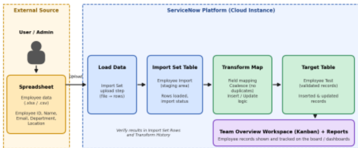
Figure 1: Architecture and data flow of the spreadsheet import using Import Sets and Transform Maps
